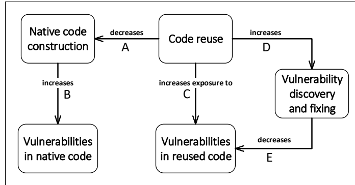
Figure 1: Theoretical model.
