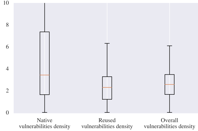
Figure 3: Boxplots of vulnerability density in native code (left), reused code (center), and overall (right)
