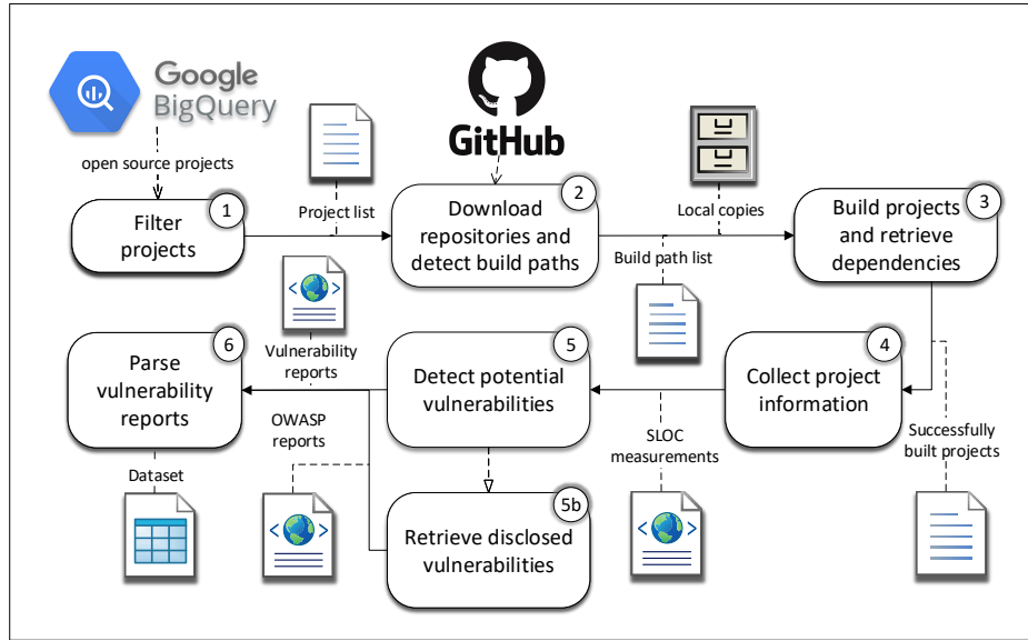
Figure 2: The dataset construction procedure.
